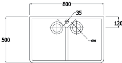
RF0800* £541.00 EXT - 800 x 500 x 220 mm WASTE - KSC7 x 2
