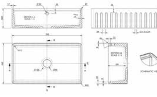
NEW BUF18132 £708.00 Butler Sink Single Bowl with Chopping Board and Grid, Fluted Front EXT - 795 x 460 x 220 mm Sit On WASTE - KSC1
