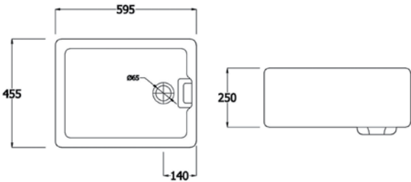
Standard Belfast £378.00 RB0001 Metric (Domestic Quality) EXT - 595 x 455 x 250 mm WASTE - KSC6 (Only available in a Stainless Steel or Non-Tarnish Brass finish)
