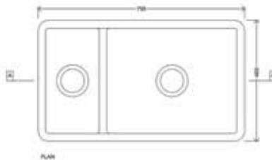
LAN1.5WHFLUTE £1134.00 Fully reversible EXT - 795 x 465 x 220 mm WASTE - KSC7 x 2
