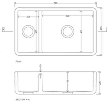
LAN1.5WH £1032.00 EXT - 795 x 465 x 220 mm WASTE - KSC7 x 2
