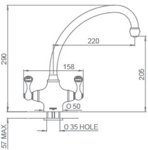
WHITEWELL FTTP0011 CHROME £474.24 SPECIAL PRICE £237.12 Monobloc sink mixer with porcelain levers and Shaws ceramic hot and cold undices, 1/4 turn ceramic valves and extended length flexible tail pipes for easy installation. Minimum 0.2 bar pressure required.
